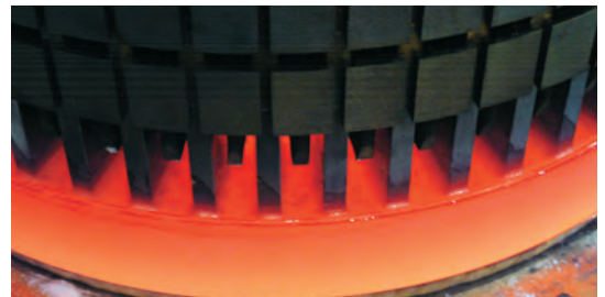
Short-circuiting ring at 780 °C
