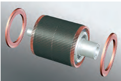
Short-circuiting ring brazing inductor
